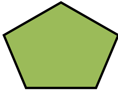
Regular Pentagon
